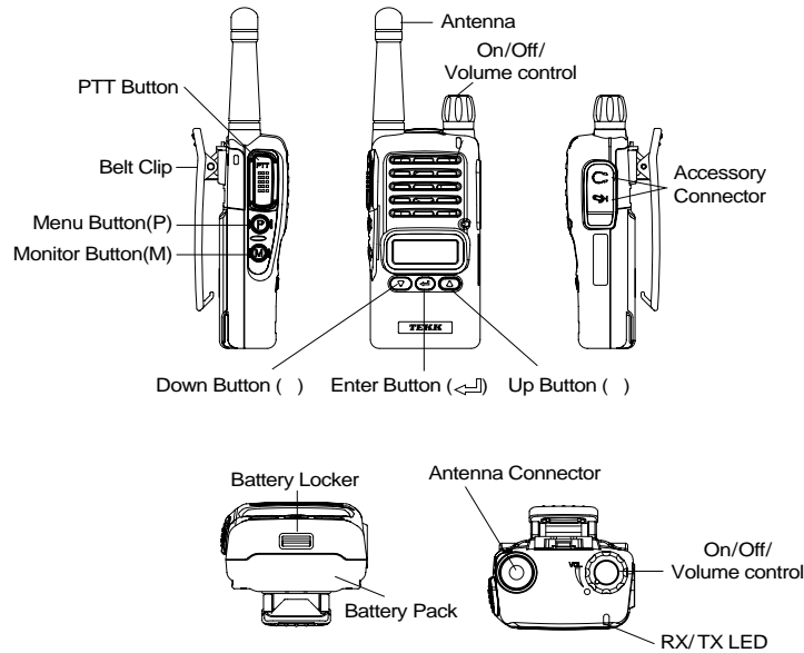
figure 3-1) Appearance of XU/XV-100 Series Radio
