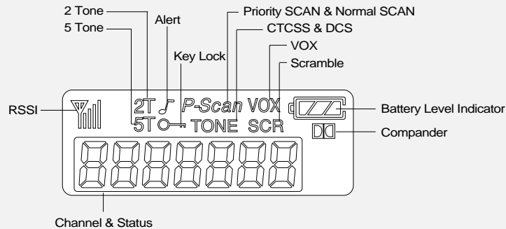
figure 3-2) XU/XV-100 Series LCD Indication
