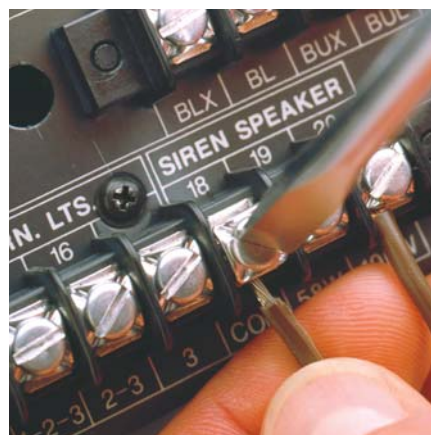
All connections are plainly labeled to speed installation.
